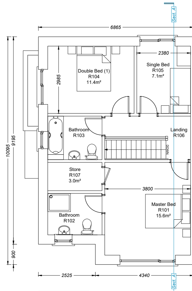
HOUSE TYPE: J FIRST FLOOR PLAN - 56.3M 2
