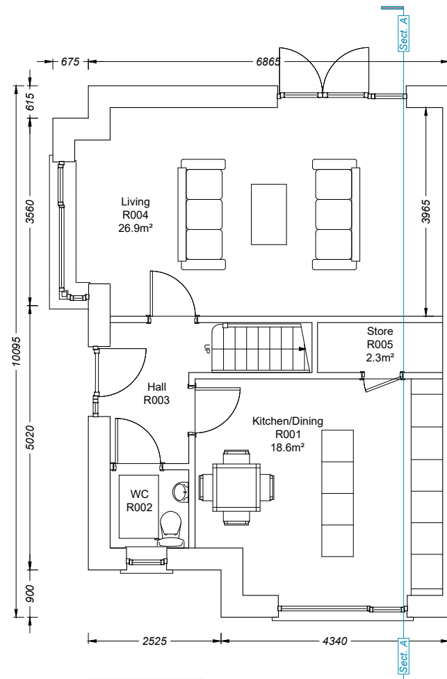
HOUSE TYPE: J GROUND FLOOR PLAN - 58.2M 2
