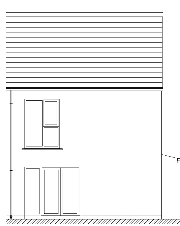
HOUSE TYPE: J REAR ELEVATION
