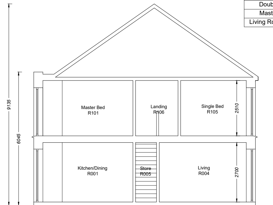
HOUSE TYPE: J SECTION AA
