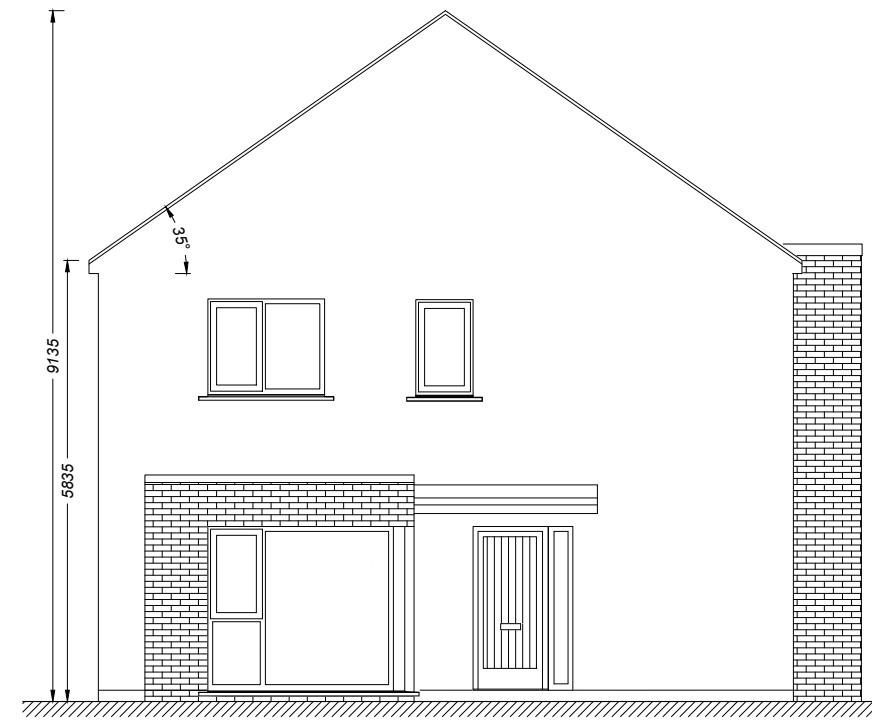
HOUSE TYPE: J SIDE ELEVATION
