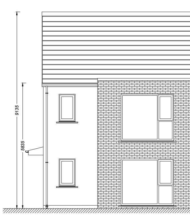
HOUSE TYPE: J FRONT ELEVATION
